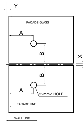
PLAN OPTION-1 (GLASS TO WALL GAP)
