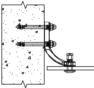
PLAN OPTION-1 (GLASS TO WALL GAP)
