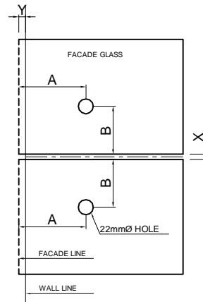
PLAN OPTION-2 (GLASS INSERTED INTO THE WALL)
