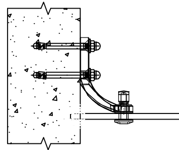
PLAN OPTION-2 (GLASS INSERTED INTO THE WALL)
